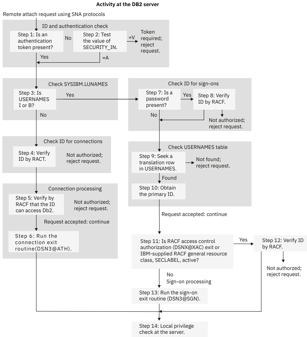
Figure 8. Db2 processing of remote attachment requests
