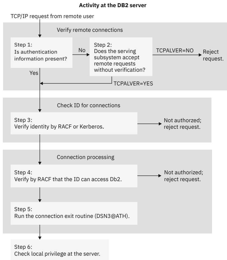
Figure 9. Db2 processing of TCP/IP-based connection requests
