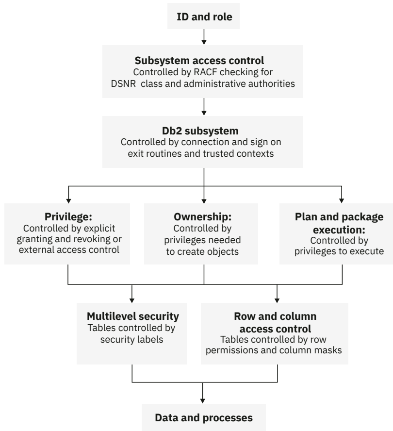
Figure 2. Access to objects and data within Db2
