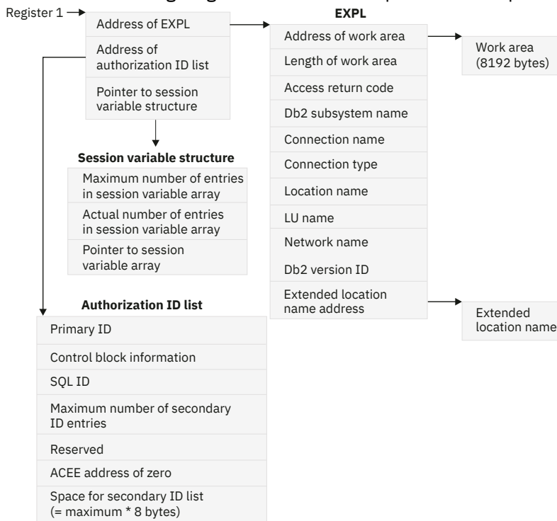
Figure 13. How a connection or sign-on parameter list points to other information
