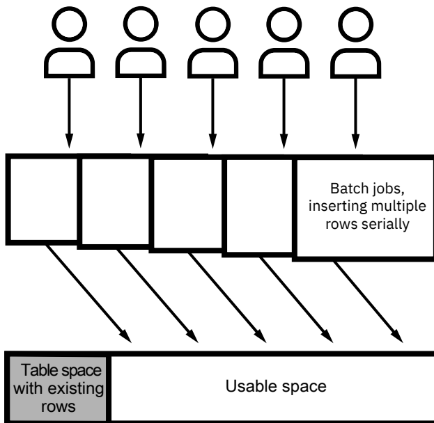
Figure 7. A small number of batch jobs each inserting multiple rows serially might not experience a performance improvement from IAG2.
