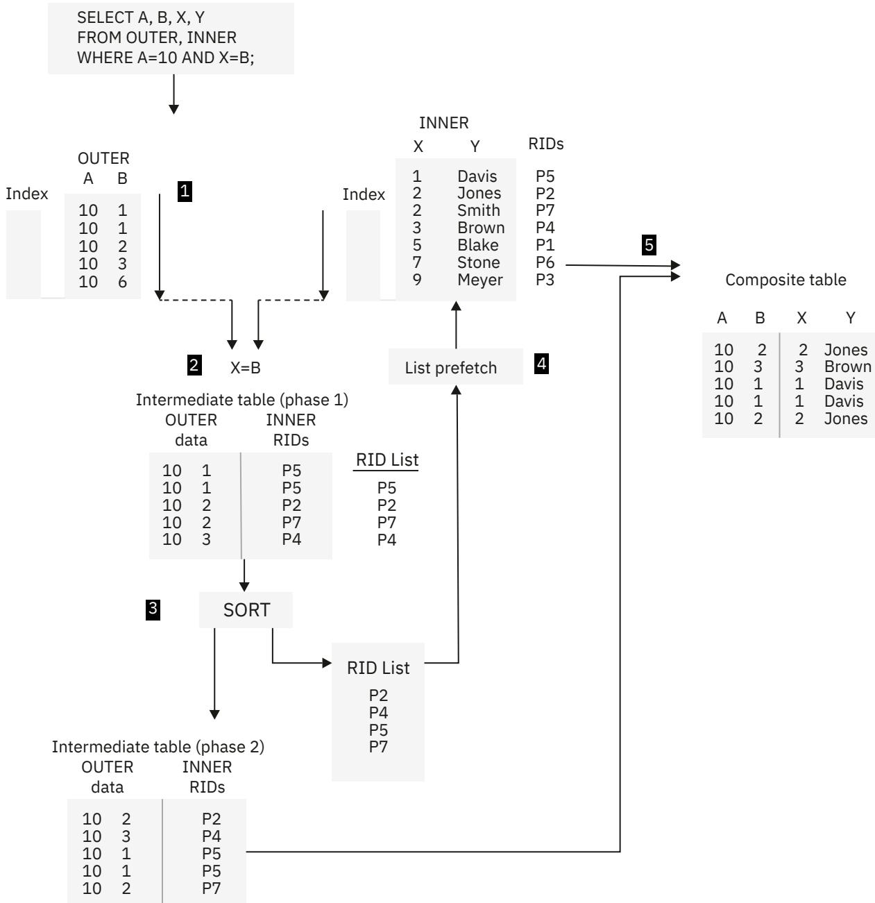
Figure 52. Hybrid join (SORTN_JOIN='Y')
