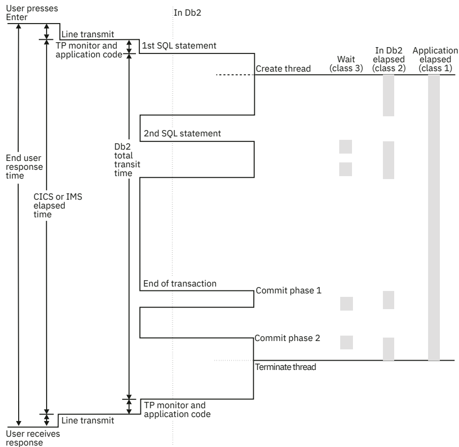
Figure 46. Transaction response times
