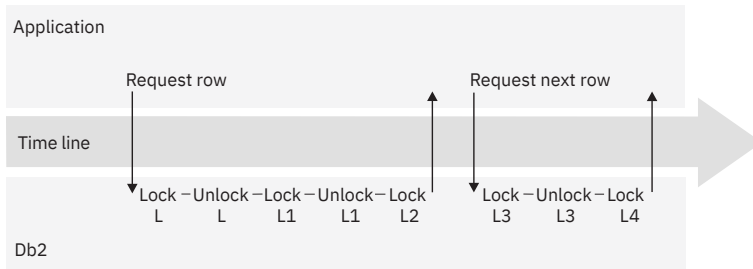
Figure 18. How an application that uses RS isolation acquires locks when no lock avoidance techniques are used
