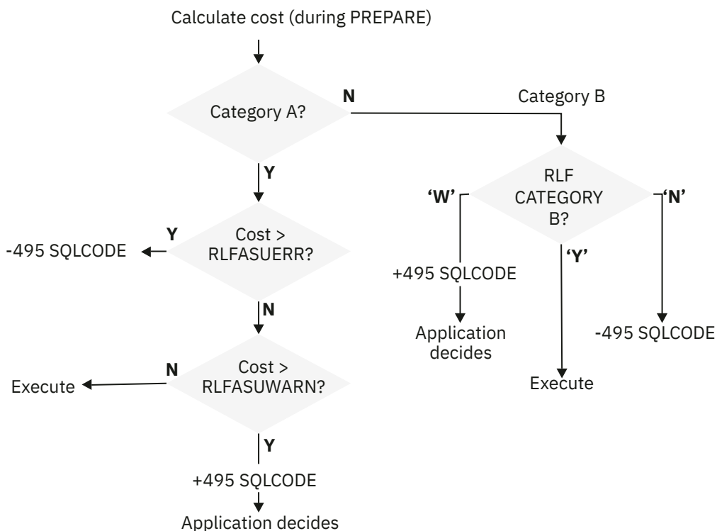
Figure 10. Processing for predictive governing
