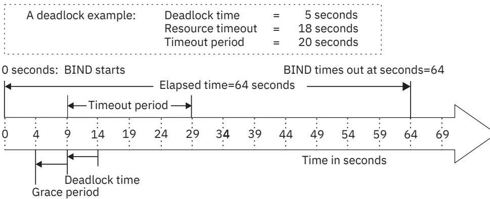
Figure 2. An example of scanning for timeout
