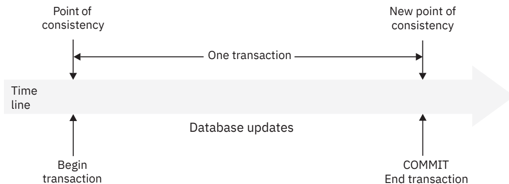
Figure 46. A transaction with a commit operation
