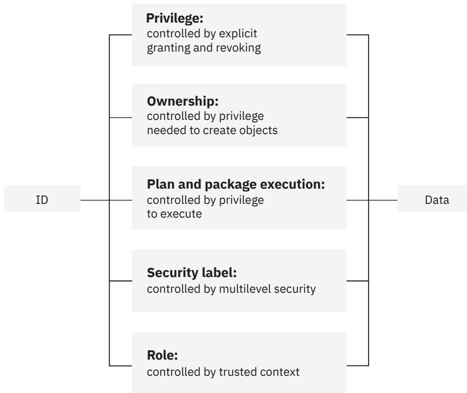
Figure 44. Granting access to data within Db2
