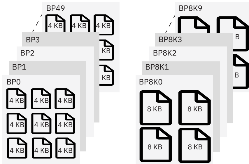
Figure 49. Buffer pools with 4 KB and 8 KB pages
