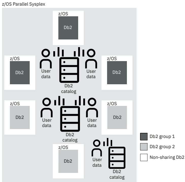
Figure 33. A possible configuration of Db2 data sharing groups
