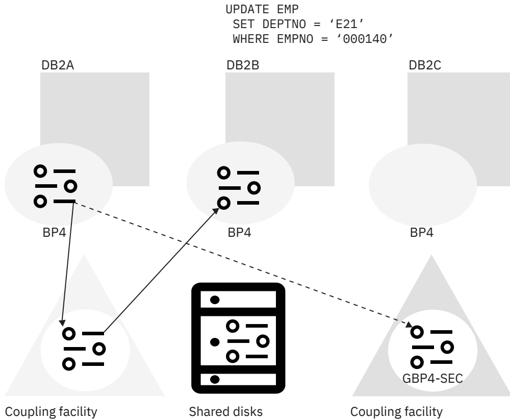
Figure 38. How DB2B updates the same data page
