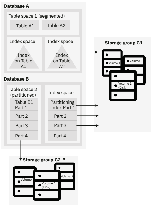
Figure 15. Hierarchy of Db2 structures
