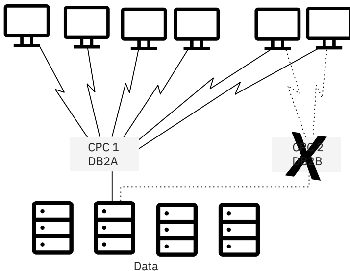
Figure 31. How data sharing improves availability during outages
