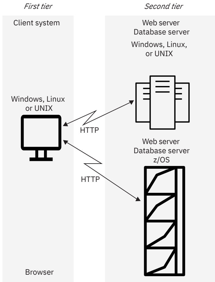
Figure 53. Two-tier connectivity between a workstation-based client and different database servers
