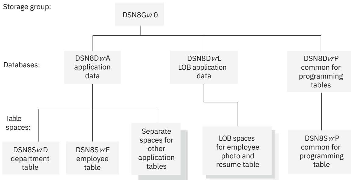
Figure 72. Relationship among sample databases and table spaces
