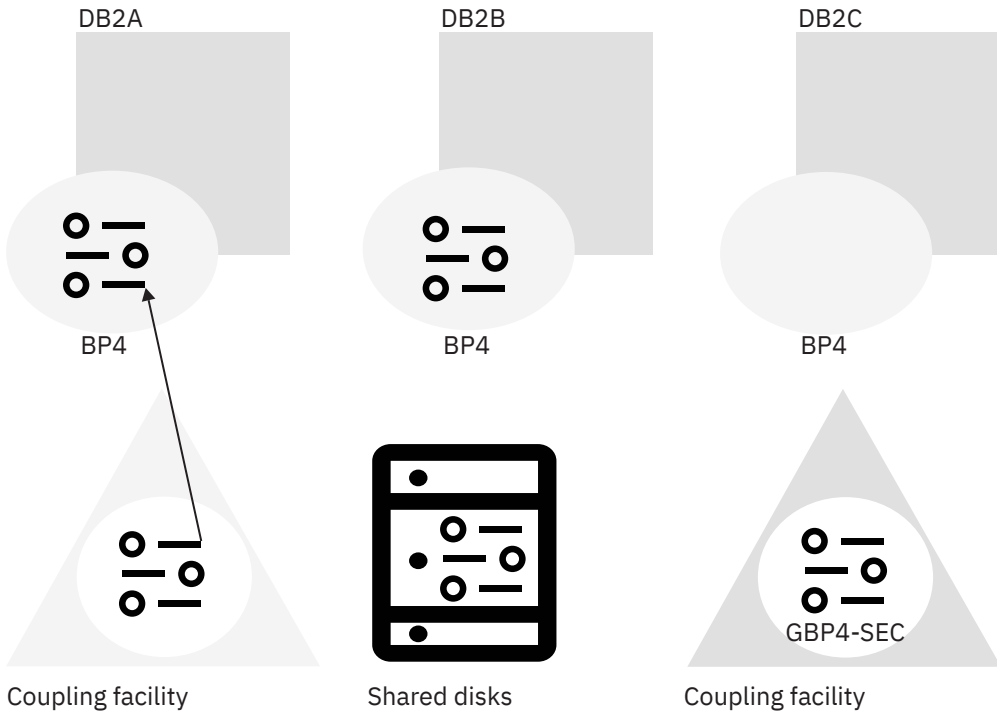
Figure 40. DB2A reads data from the group buffer pool
