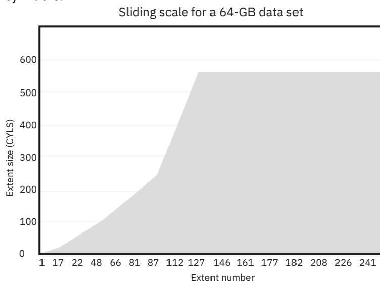
Figure 11. Sliding scale allocation of secondary extents for a 64 GB data set
