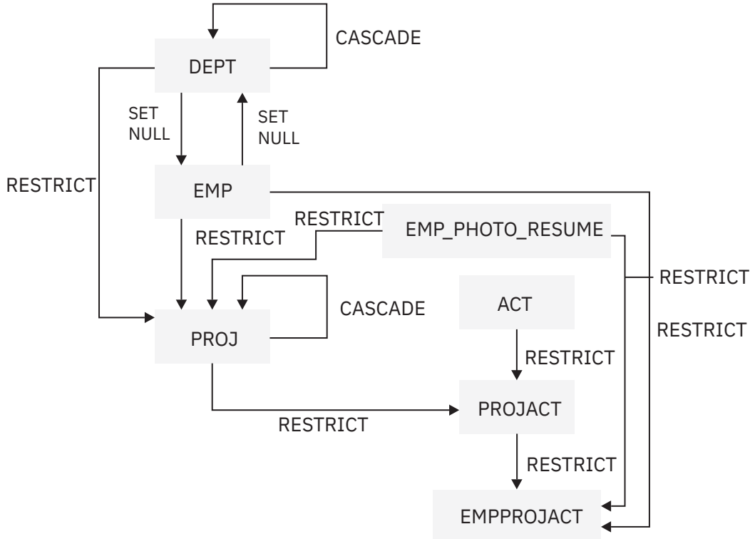
Figure 70. Relationships among tables in the sample application
