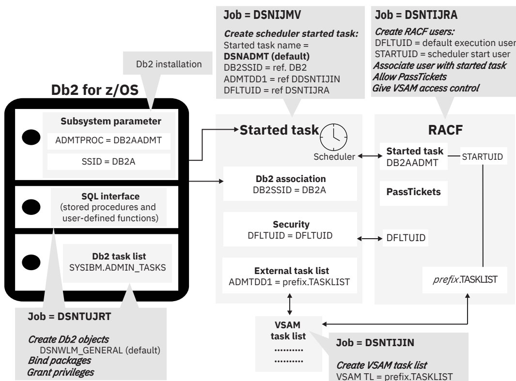
Figure 78. Setting up the administrative task scheduler
