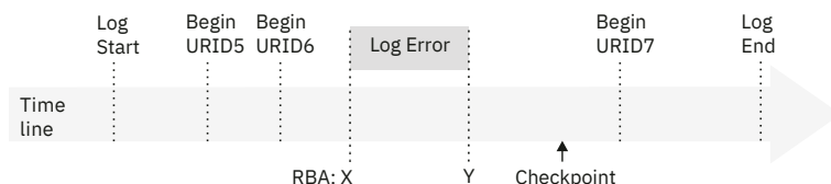
Figure 58. Illustration of failure during backward log recovery
