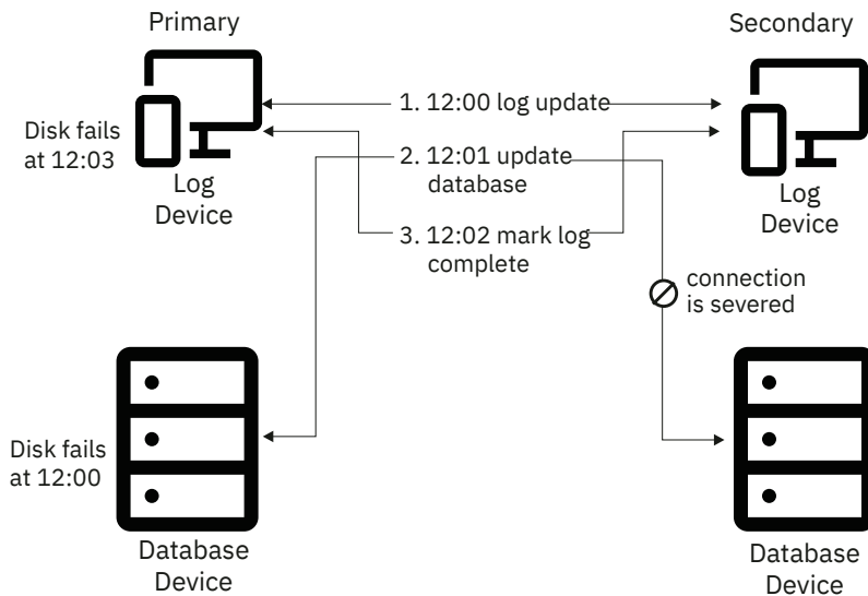
Figure 59. Data inconsistency caused by a rolling disaster
