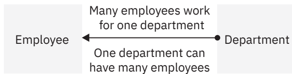
Figure 2. Assigning many-to-one facts to an entity
