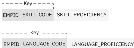
Figure 10. Entities that satisfy the fourth normal form
