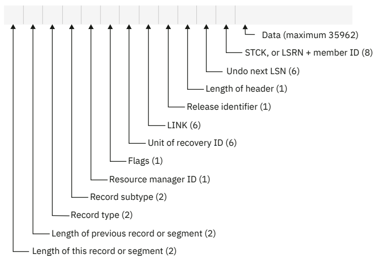
Figure 69. 6-byte format of a Db2 recovery log record
