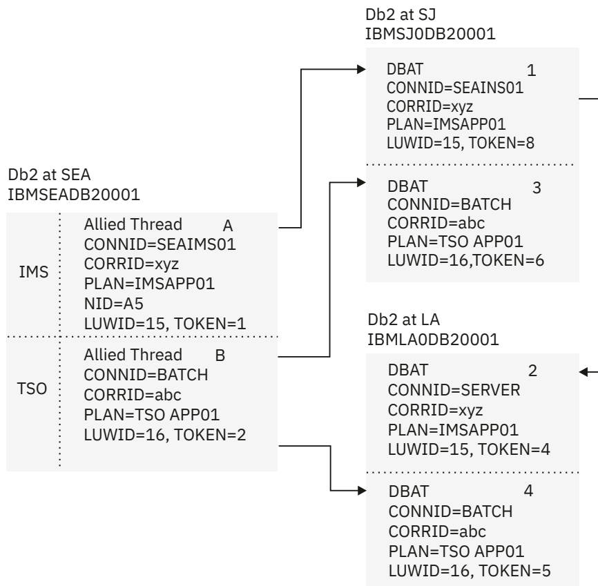
Figure 65. Resolution of indoubt threads
