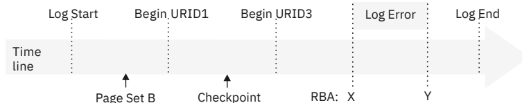
Figure 54. Failure during current status rebuild
