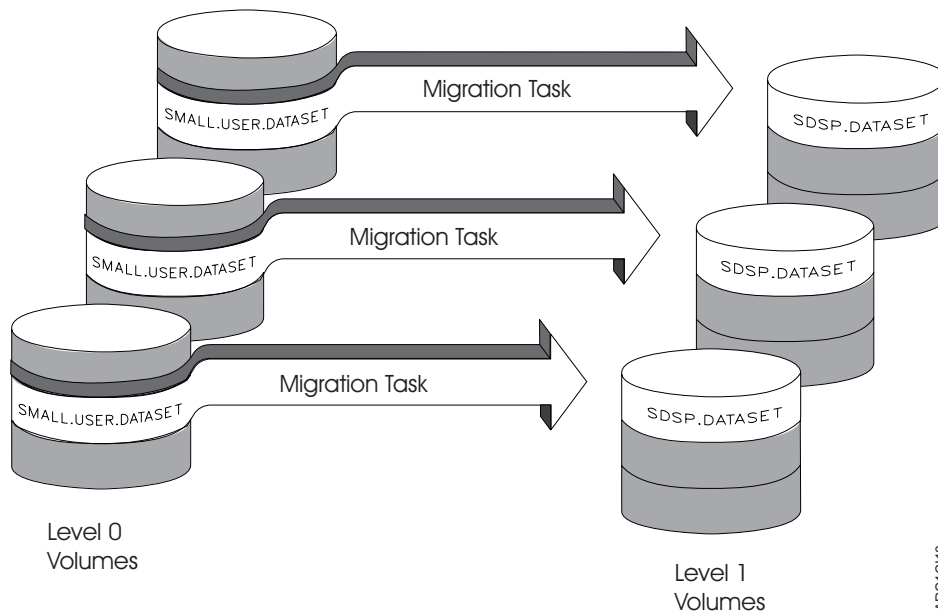
Figure 12. Part 1—Ideal Multitasking Migration. Three migration tasks migrate three small user data sets to three level-1 migration volumes on which SDSP data sets are defined.
