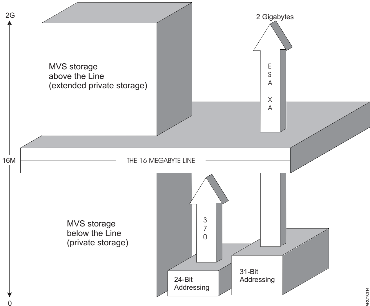
Figure 83. The MVS Storage Environment
