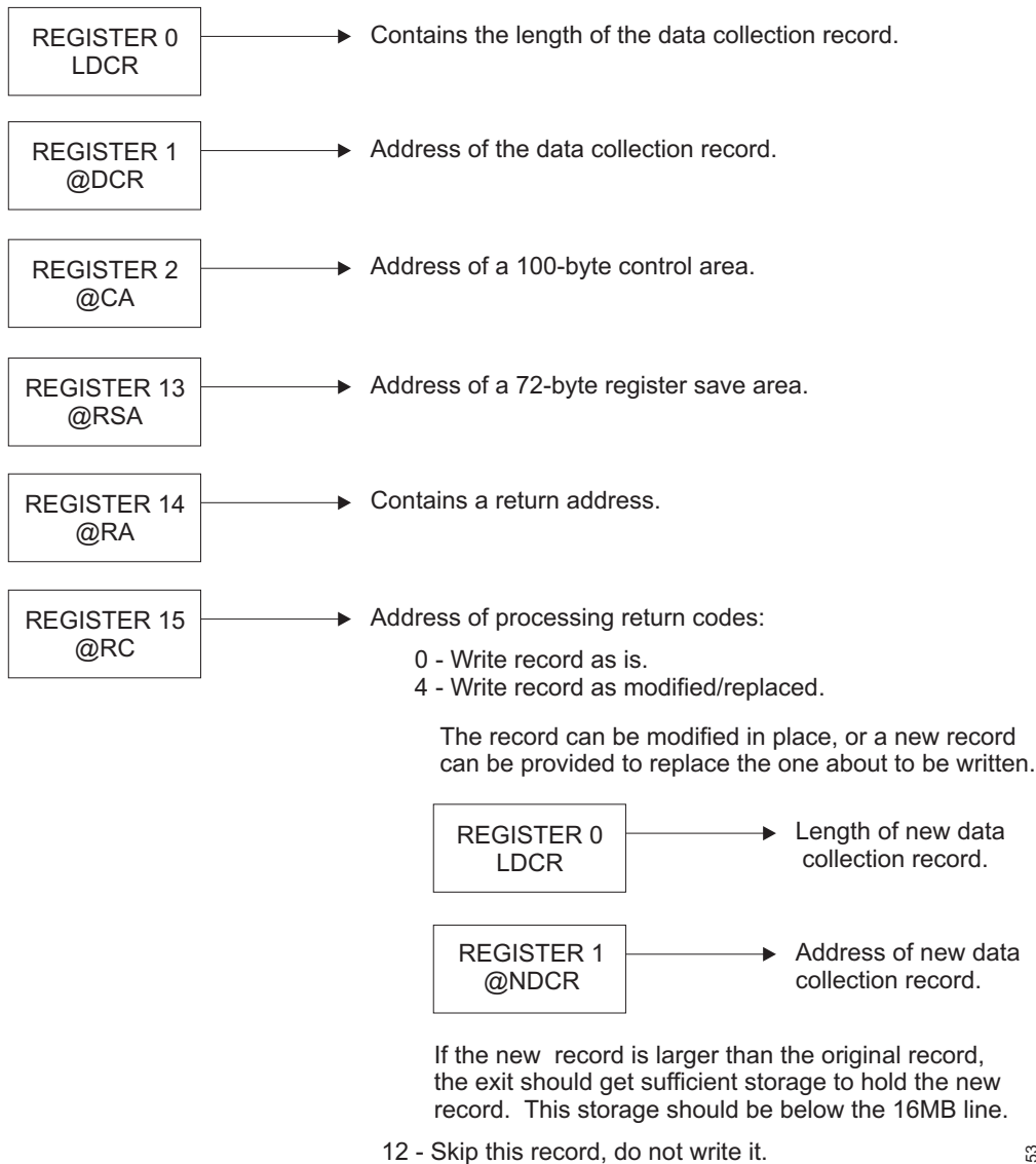
Figure 99. Exit for Data-Collection Support
